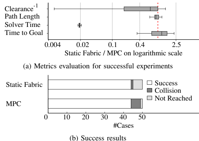
Fig. 7: Results for randomized motion planning problems with the panda robot in simulation. Lower values represent an improved performance of SF over MPC.
